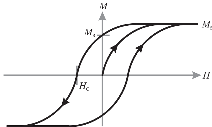
Figure 13.3. A hysteresis loop.
