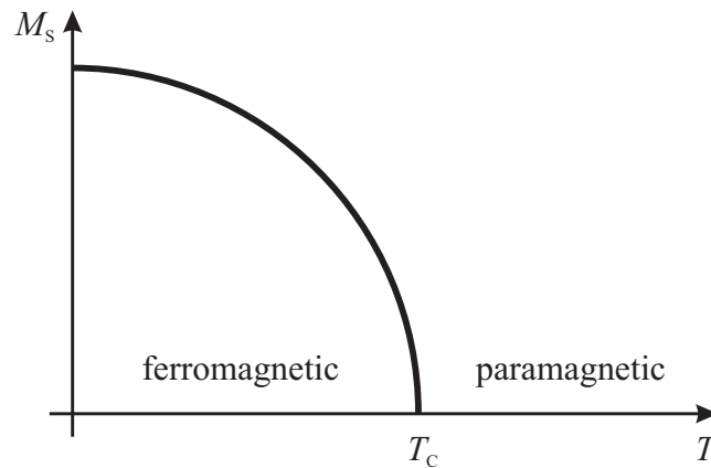
Figure 13.4. The temperature dependence of the saturation magnetization.
