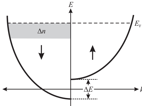
Figure 13.2. Spin band splitting in a field.
