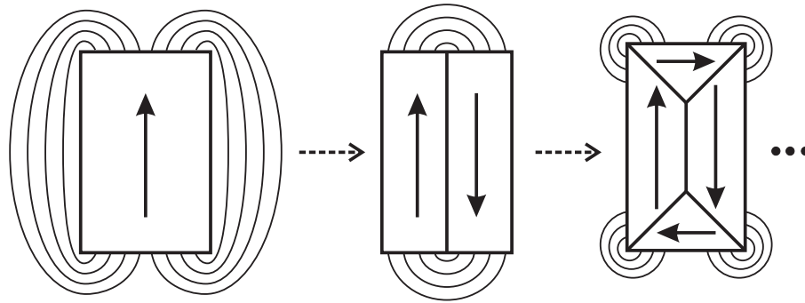
Figure 13.5. Magnetic domains reduce return flux energy.
