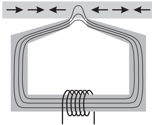
Figure 13.6. An inductive recording head.
