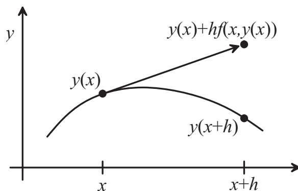
Figure 8.1. An Euler method.
