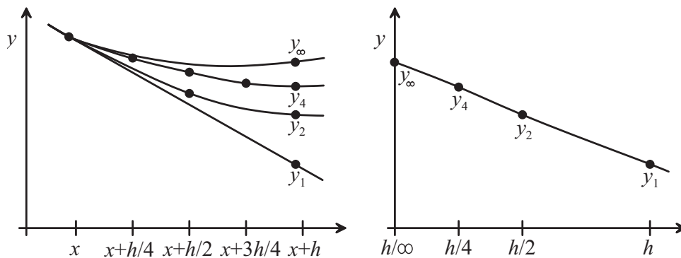
Figure 8.4. Richardson extrapolation.
