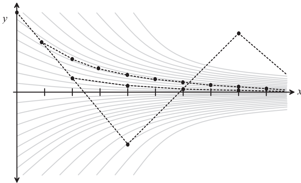
Figure 8.2. Origin of oscillation in the Euler method. The gray lines show the family of solutions of dy/dx = Ay , and the dotted lines show the numerical solution for various step sizes. Figure 8.2 shows why the Euler method is such a poor approximation.
