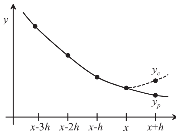
Figure 8.3. A predictor-corrector method.
