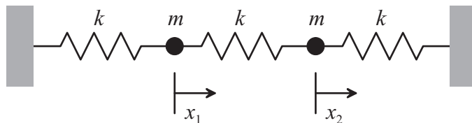
Figure 4.2. Two coupled harmonic oscillators.
